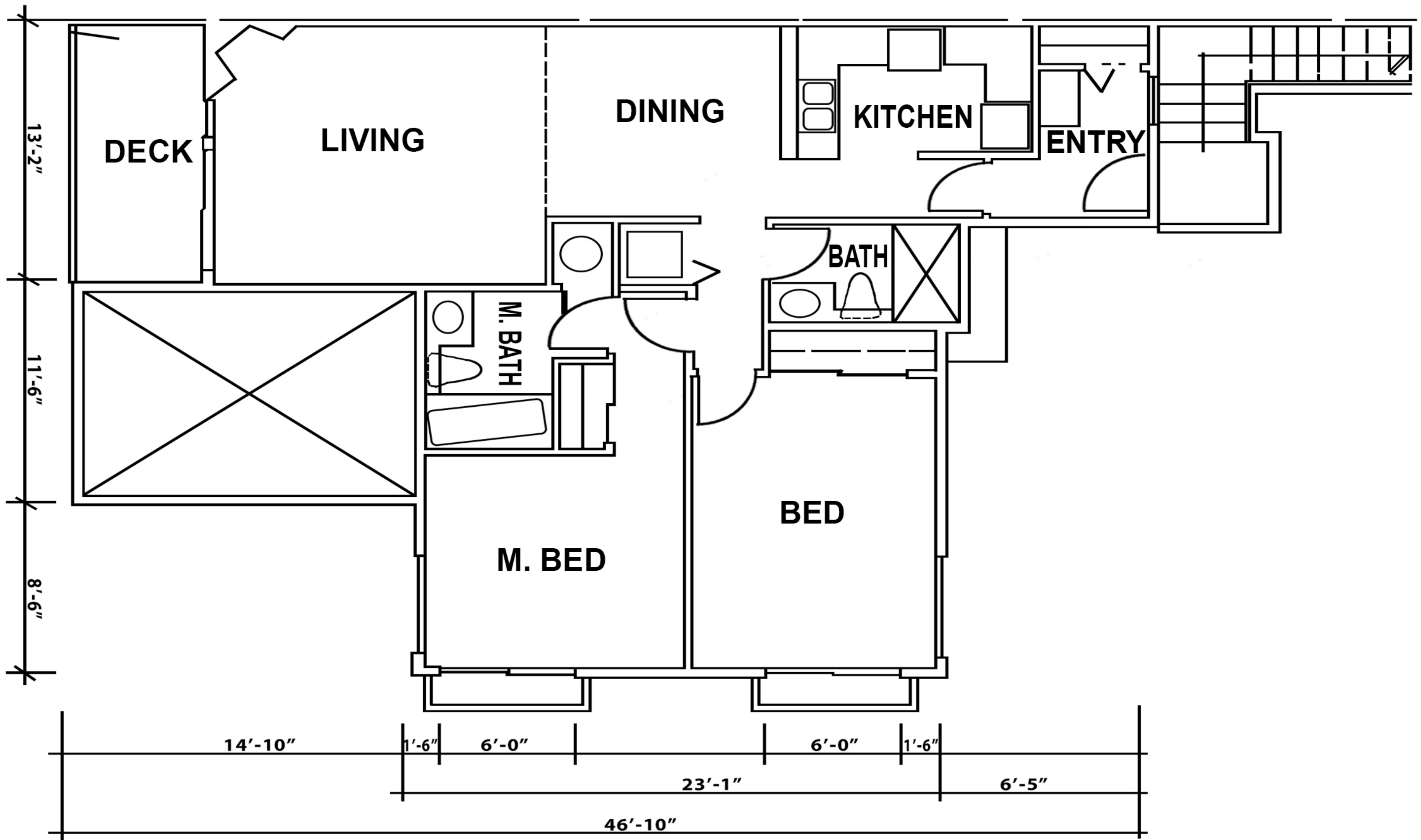
PLAN E (SECOND FLOOR)
